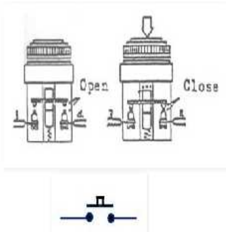
Gambar 5. Push Button
